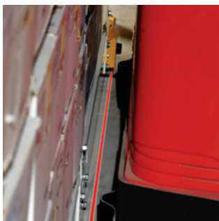
A Photo Sweep® stretches the full length of each carriage side for end-to-end safety.
